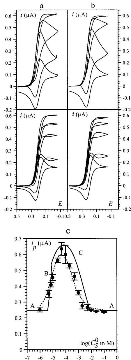
Figure 2. (a) Cyclic voltammograms (scan rate: 50 \text{ mV s}^{-1} ) recorded in a phosphate buffer solution (pH 7.4) containing 20 \mu\text{M} [\text{Os}(\text{bpy})_2\text{pyCl}]^{2+} , 0.2 \mu\text{M} HRP, and increasing concentrations of \text{H}_2\text{O}_2 (upper curves, from bottom to top, 0, 0.01, 0.025, 0.05 mM; lower curves, from top to bottom, 0.1, 0.2, 0.5, 25 mM). The scan is started ca. 20 min after mixing the reactants (see text). (b) Corresponding simulated curves (for details, see text). E in volts vs SCE. (c) Variation of the peak or plateau (when there is no peak) current with the concentration of \text{H}_2\text{O}_2 . Filled circle symbol: experimental average value of 3–10 measurements per data. The vertical bars are the standard deviations. Full lines: theoretical curves in the case of (A) absence of catalysis; (B) control by \text{H}_2\text{O}_2 diffusion (total catalysis); (C) plateau current according to eq 6. Dotted line: finite difference simulation.
