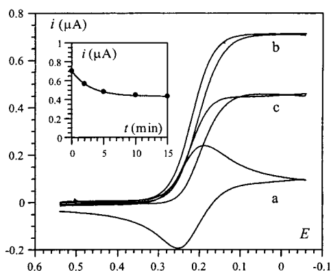
Figure 5. Cyclic voltammograms obtained at 50 \text{ mV s}^{-1} in a phosphate buffer (pH 7.4) containing (a) 20 \mu\text{M} [\text{Os}(\text{bpy})_2\text{pyCl}]^+ alone; (b,c) 20 \mu\text{M} [\text{Os}(\text{bpy})_2\text{pyCl}]^+ , 0.2 \mu\text{M} HRP, and 0.2 \text{ mM} \text{H}_2\text{O}_2 . The curve was recorded (b) immediately after the addition of the three components and (c) after an incubation time of 15 min. Inset: dependence of the plateau current on the incubation time.
