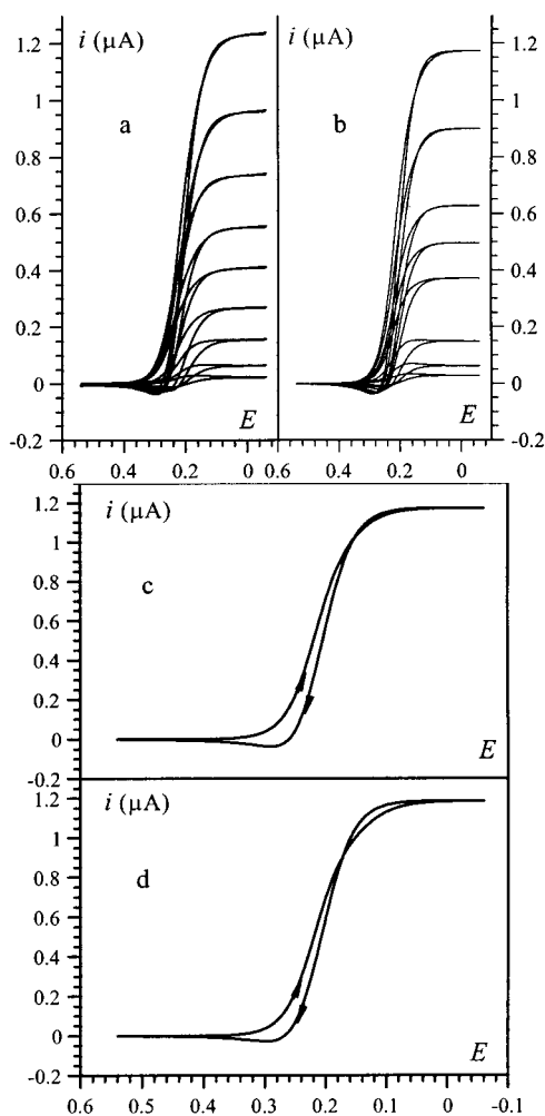
Figure 11. (a) Cyclic voltammograms (scan rate: 10 mV/s) recorded (after attainment of steady state before starting the potential scan) in a phosphate buffer solution (pH 7.4) containing 25 mM H 2 O 2 , 0.2 μM HRP, and increasing concentrations of [Os(bpy) 2 pyCl] 2+ . From bottom to top: 5, 10, 20, 30, 40, 50, 60, 80, 100 μM. (b) Simulated curves obtained with k_1 = 1.7 \times 10^7 \text{ M}^{-1} \text{ s}^{-1} , K_{1,M} = 128 \text{ μM} , k_2 \gg k_1 , k_3 = 1.4 \times 10^7 \text{ M}^{-1} \text{ s}^{-1} , K_{3,M} = 20 \text{ μM} , k_4 = 55 \text{ M}^{-1} \text{ s}^{-1} , k_5 = 1900 \text{ M}^{-1} \text{ s}^{-1} , k_6 = 0.012 \text{ s}^{-1} . (c) Simulated curve for 100 μM cosubstrate with the same values of the kinetic characteristics as in (b). (d) As in (c), except that the values of k_4 , k_5 , and k_6 have been lowered by 30%, keeping constant the ratios k_4/k_5 and k_6/k_5 .
