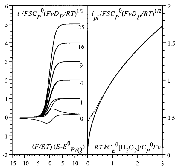
Figure 1. Cyclic voltammetry of a standard catalytic mechanism where the rate-determining step (rate constant: k ) is first order in \text{H}_2\text{O}_2 (top scheme). (a) Cyclic voltammogram obtained upon increasing the parameter RTkC_E^0/C_P^0Fv . (b) Variation of the peak (dotted line) or the plateau current (full line) with the same parameter.
