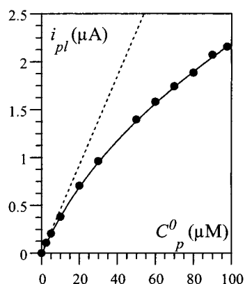
Figure 6. Catalytic plateau current as a function of the cosubstrate concentration recorded at 50 \text{ mV s}^{-1} just after mixing in a phosphate buffer (pH 7.4) containing 0.2 \mu\text{M} HRP and 0.2 \text{ mM} \text{H}_2\text{O}_2 . Full line: fitting with a Michaelis–Menten kinetics according to eq 6. Dotted line: low concentration linear variation (eq 7).
